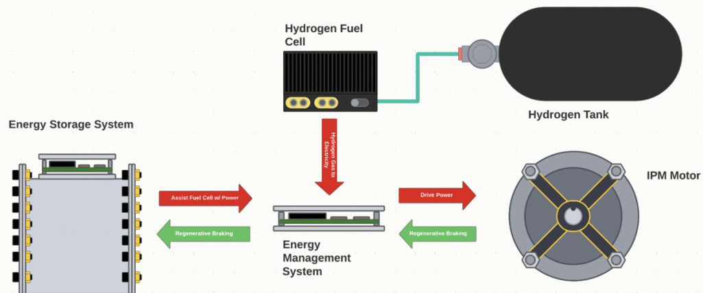
MIT Electric Vehicle Team Diagram of a Fuel-Cell Electric Vehicle
